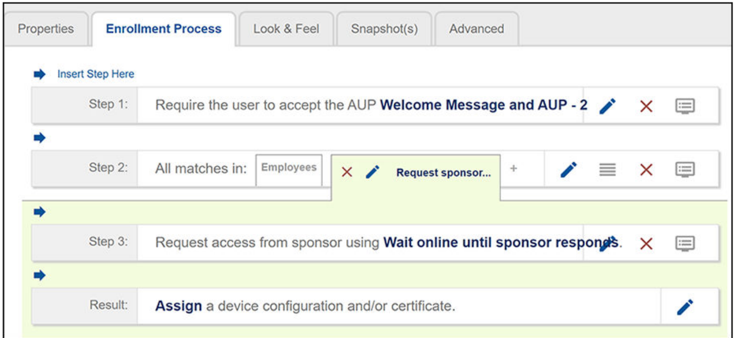
FIGURE 73 Sample Workflow That Uses the "Request Access from a Sponsor Online" Plug-in
