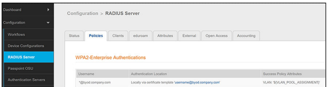
FIGURE 60 Confirming VLAN Variable in RADIUS Server Policies
