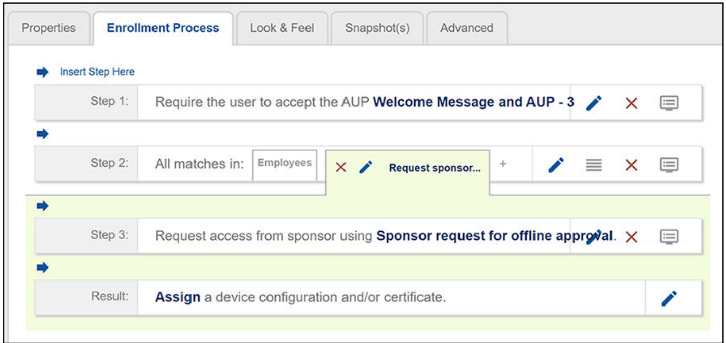
FIGURE 79 Sample Workflow That Uses the "Request Access from a Sponsor Offline" Plug-in
