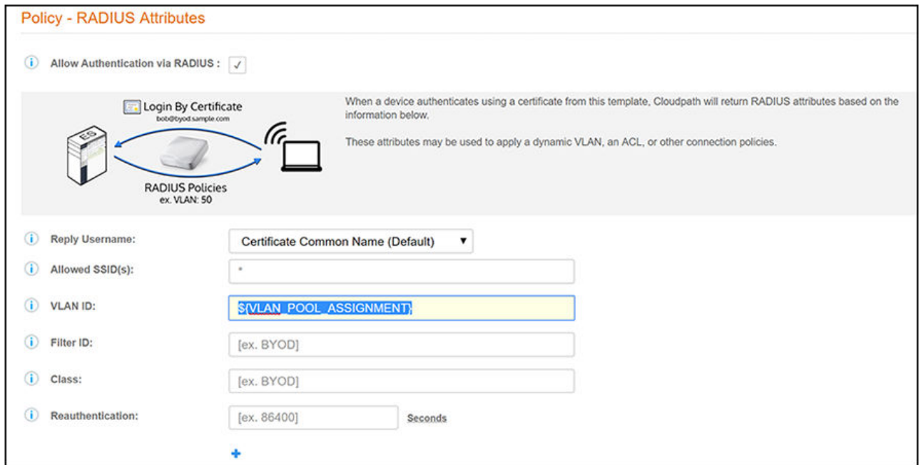
FIGURE 59 Certificate Template VLAN Variable Setting
