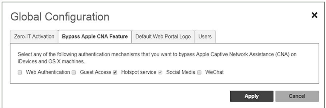
FIGURE 105 Enabling the Bypass Apple CNA Feature Globally on Unleashed
