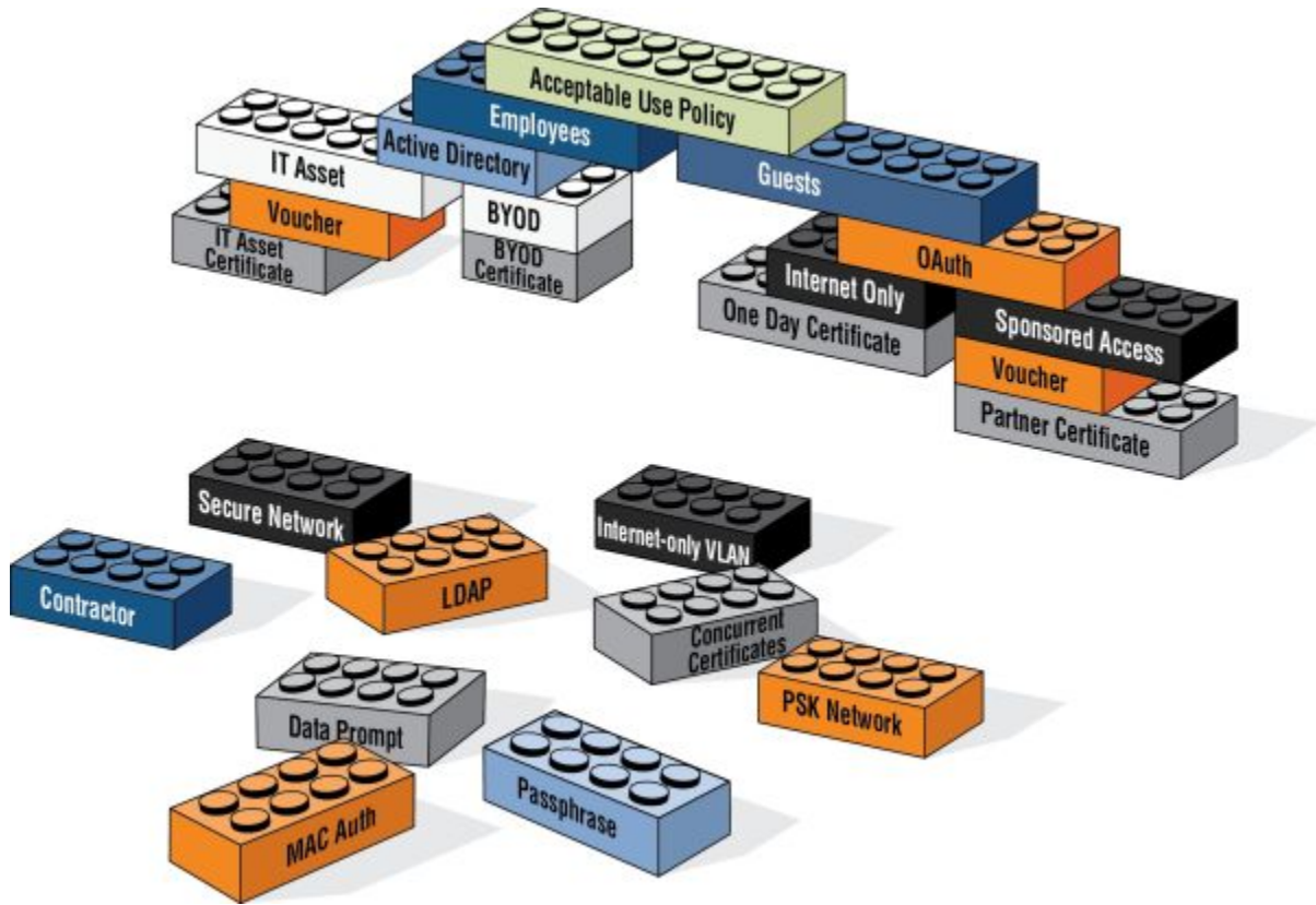
FIGURE 6 Complex Workflow
