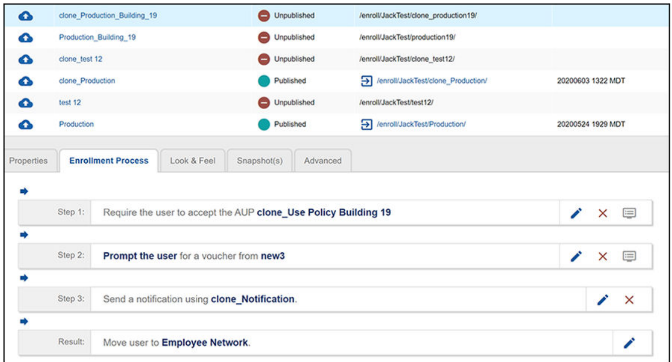
FIGURE 58 Cloned Workflow Added to Top of Workflow List
