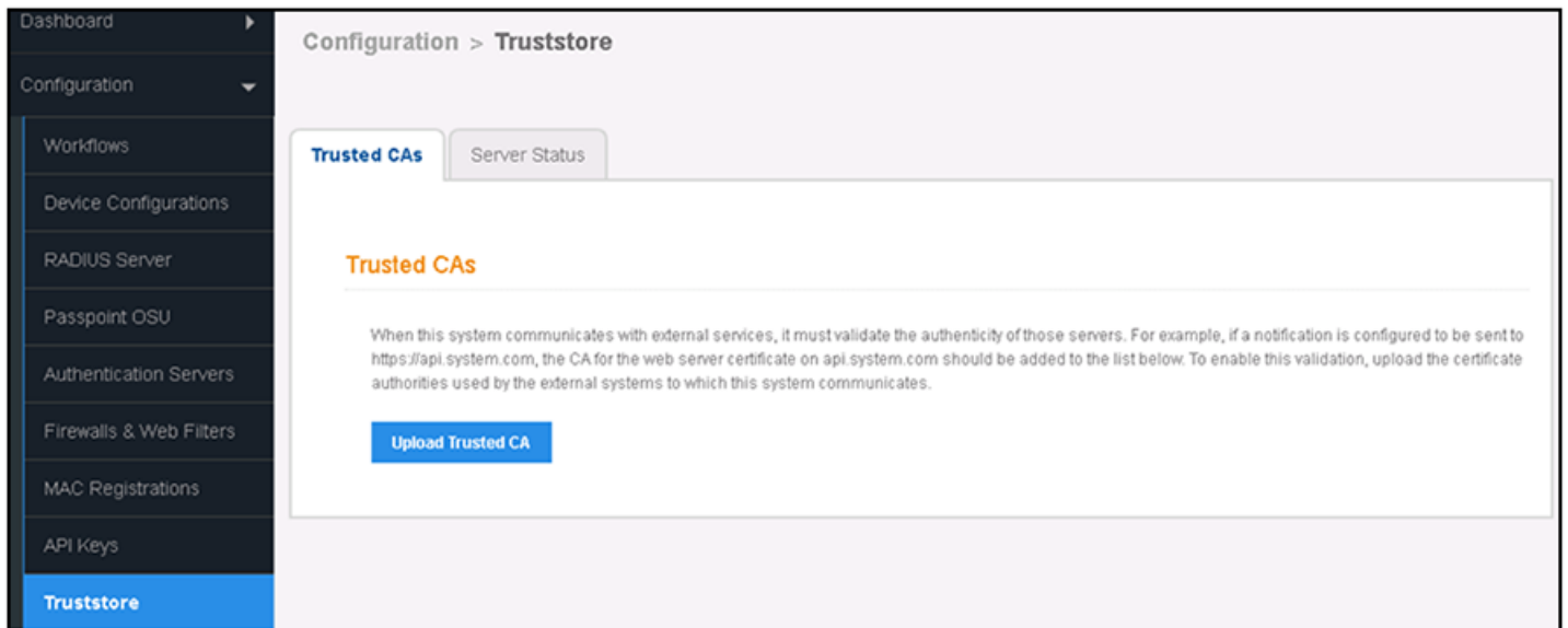
FIGURE 110 Truststore Screen Before Certificates Are Added
